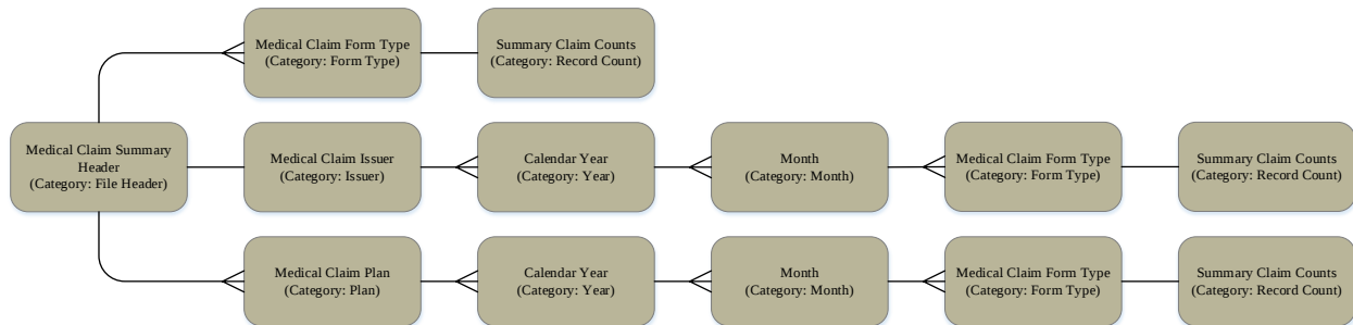
Figure 6-12: EDGE Server Summary Medical Claim File Accept – Reject Error Report (ESSMFE) Data Categories
