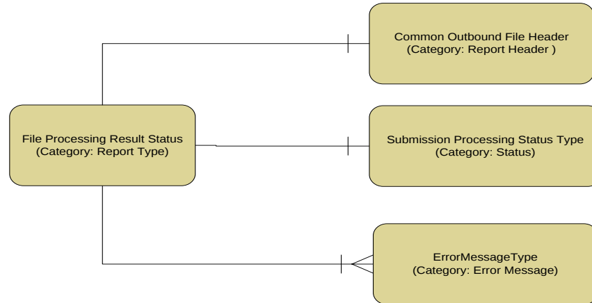
Figure 6-6: EDGE Server File Accept – Reject Report Data Categories
